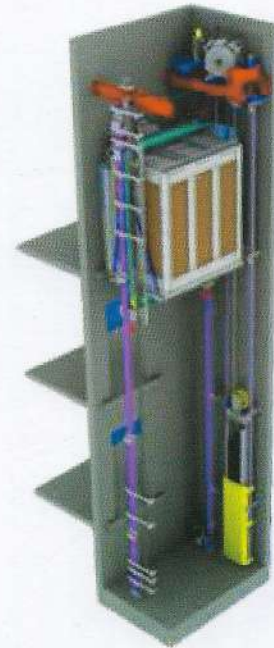
MRL Section of Hoistway
