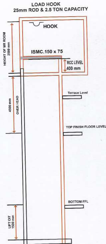
MR Section of Hoistway
