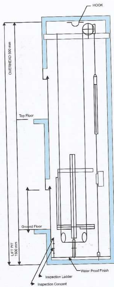
MRL Section of Hoistway
